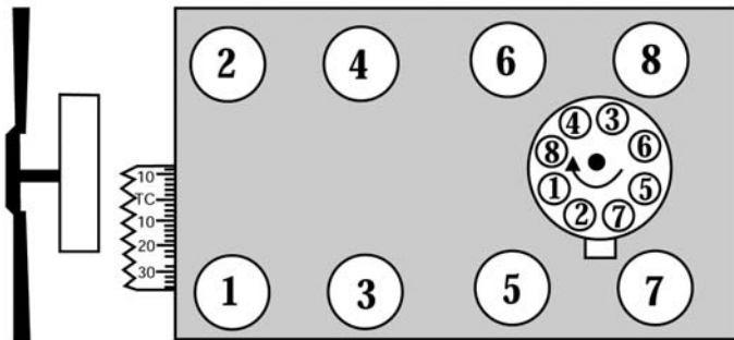
Firing Order: 1-8-4-3-6-5-7-2
